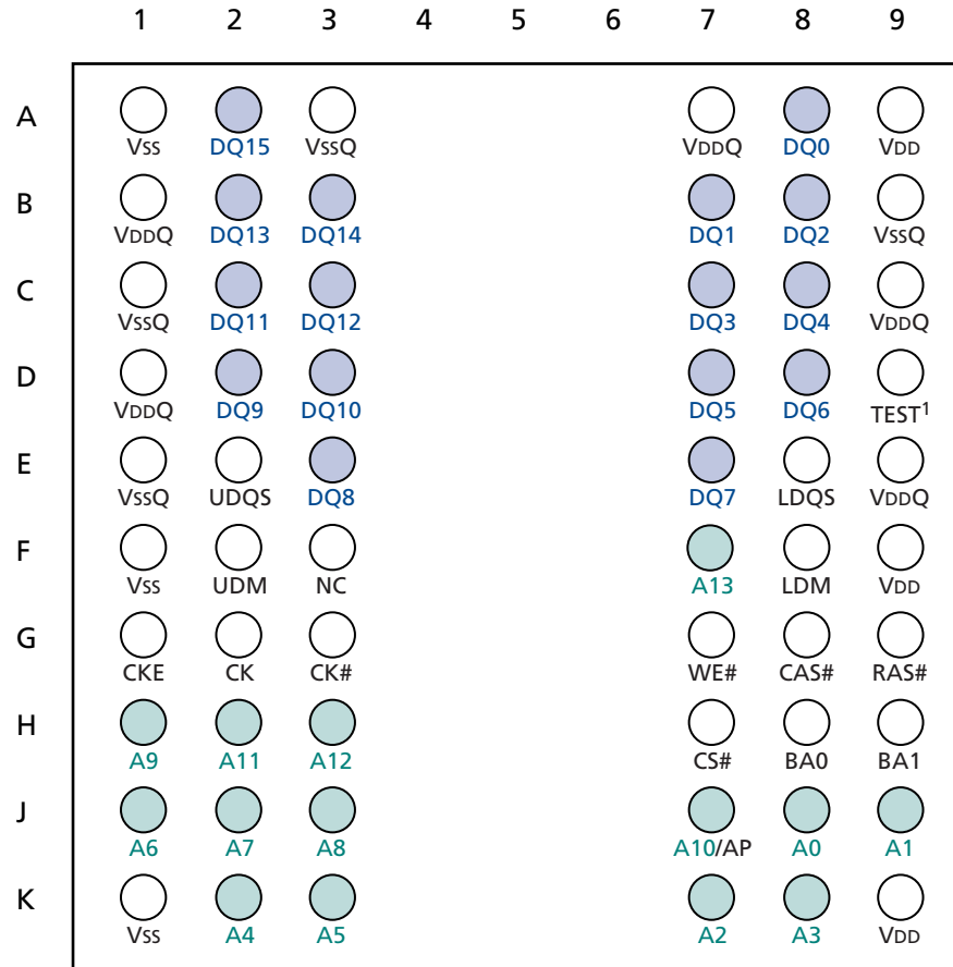
Figure 4: 60-Ball VFBGA Assignments – 10mm x 11.5mm (Top View)
